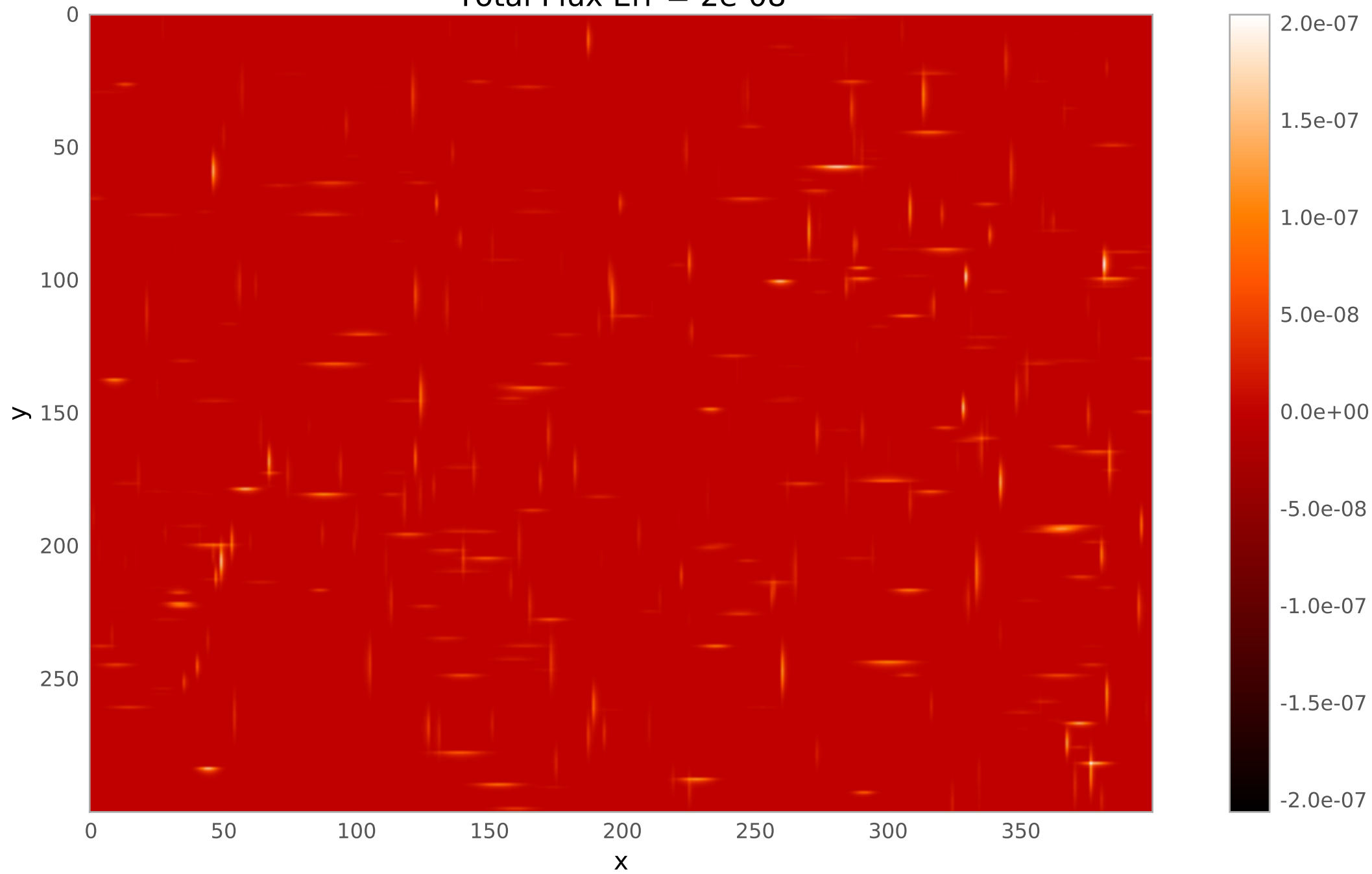
Difference Image Total Flux Err = 2e-08
