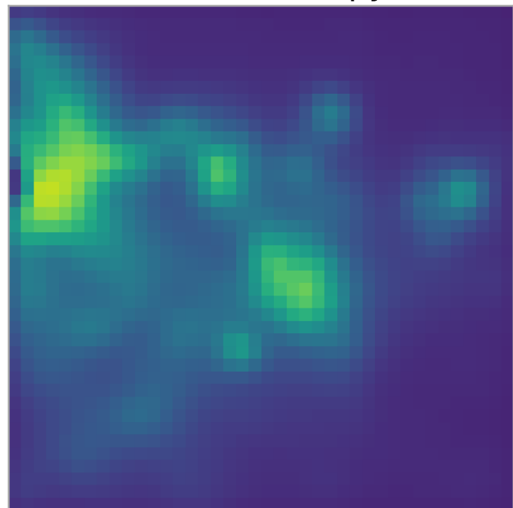
Default astropy
